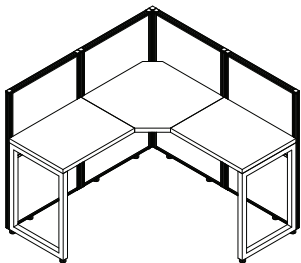
BX101M6F14-A 64"x64" L-Shape Workstation with 4 Panels Grey Tops & Fabric/Silver Frame Desk: 63"x63", 24.5"D, 29.5"H Panels: 44.5"H x 31.5"W x 1"T CU:10.6 WT: 132 lbs. List: $2195
