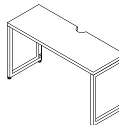
BX101M6F14-D 63"x24.5" Add-On Bench Style Workstation Grey Tops & Fabric/Silver Frame Desk: 63"W x 24.5"D x 29.5"H Panels: 44.5"H x 31.5"W x 1"T CU: 7.5 WT: 62 lbs. List: $695
